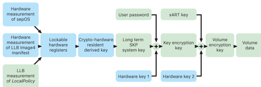
The Sealed Key Protection process.
