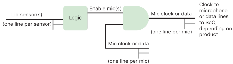
Circuit diagram.
