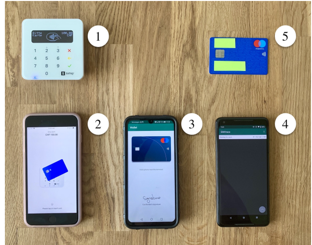
Figure 5: Setup of the testing environment for our proof-of-concept implementation, displaying the following devices: (1) SumUp Plus Card Reader, (2) mobile phone running the SumUp app and connected over Bluetooth to the SumUp reader, (3) Android phone running our app in Card Emulator mode, (4) Android phone running our app in POS Emulator mode, and (5) contactless card. Note that the device (2) is not part of the attacker’s equipment since in an actual store this device and (1) would be the payment terminal. In this scenario, the devices (3) and (4) would be the attacker’s equipment and (5) would be the victim’s card.
