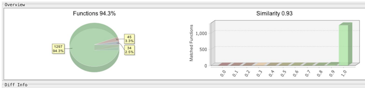
Similarity breakdown of NetHelp variants.
