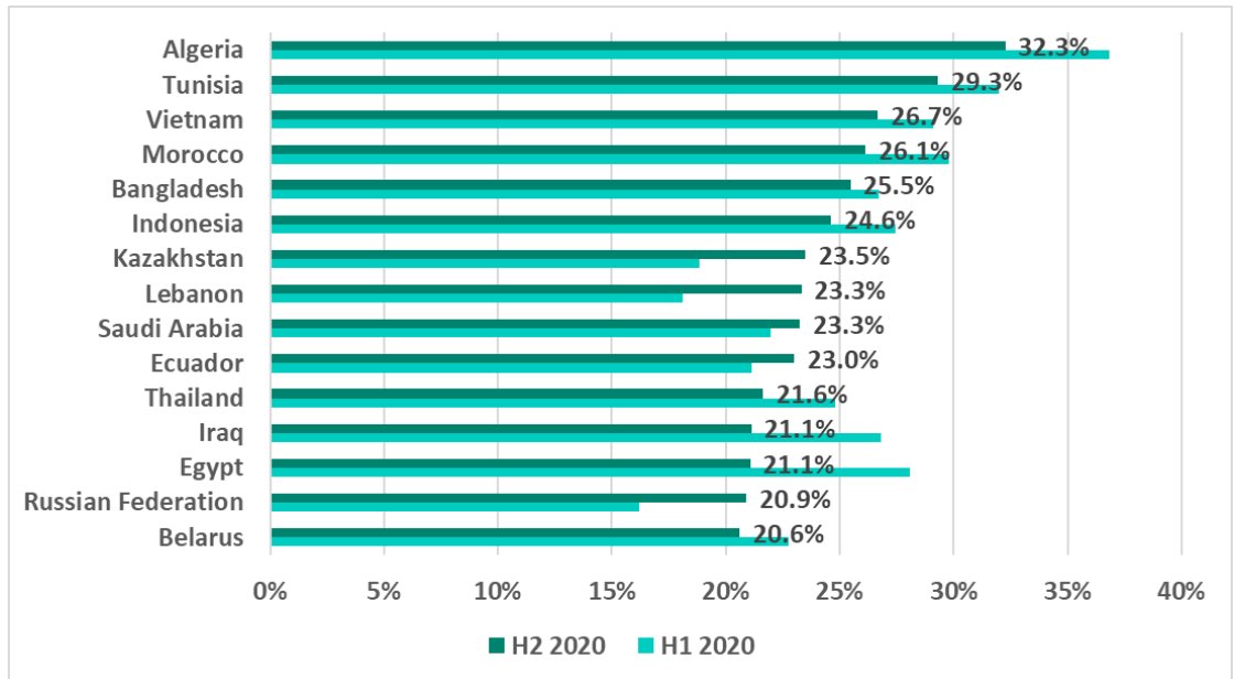
Figure 25. Top 15 countries and territories ranked by percentage of ICS computers on which threats from the internet were blocked, H2 2020
